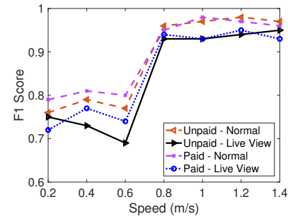
Figure 17: F1 score vs. speed.
